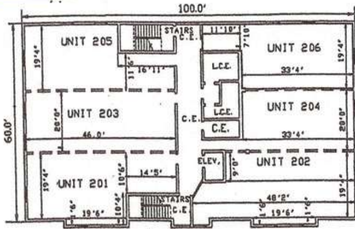
2nd FLOOR
